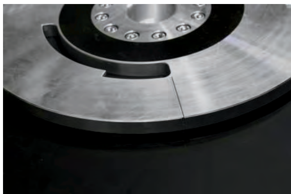
Integrated load plate
